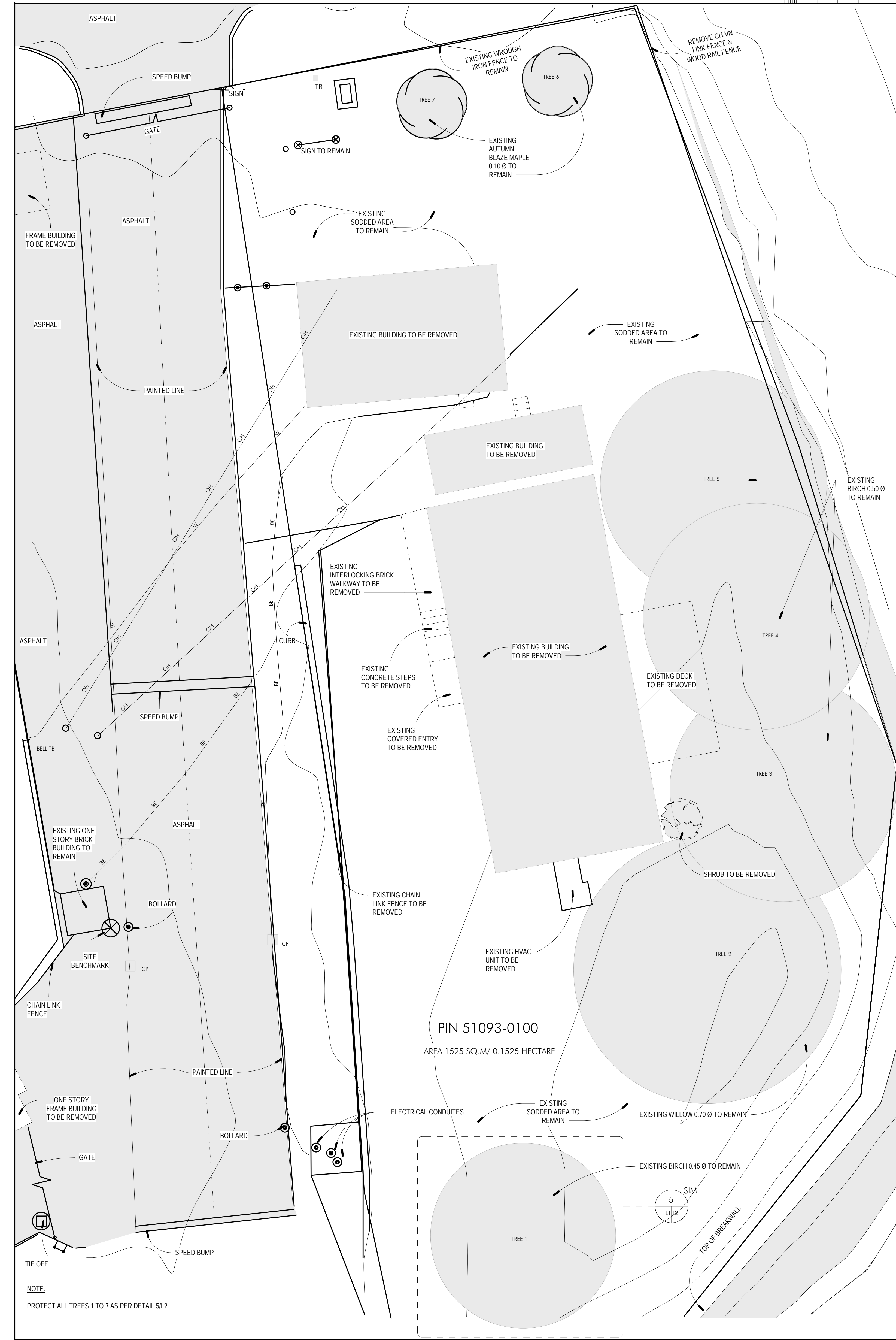
1 EXISTING SITE PLAN - SPA
